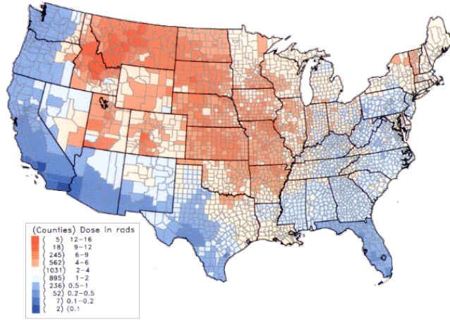
Image 1. Study Estimating Thyroid Doses of I-131 Received by Americans from Nevada Atmospheric Nuclear Bomb Test, National Cancer Institute (1997)
