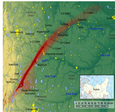
Images 2a and 2b. The Rocky Flats radioactive trace; the Kystym Urals Radioactive Trace (EURT).
